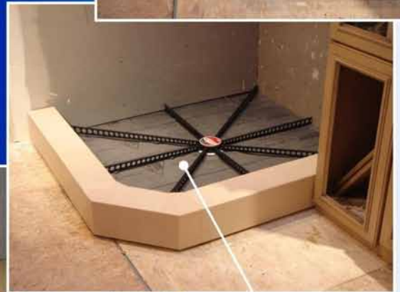
Quick Pitch® SHOWER FLOOR
